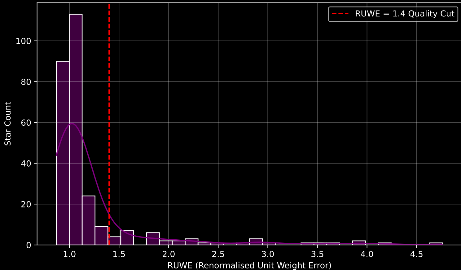
GALAH DR4 Field [307] RUWE Distribution (n= 274)
