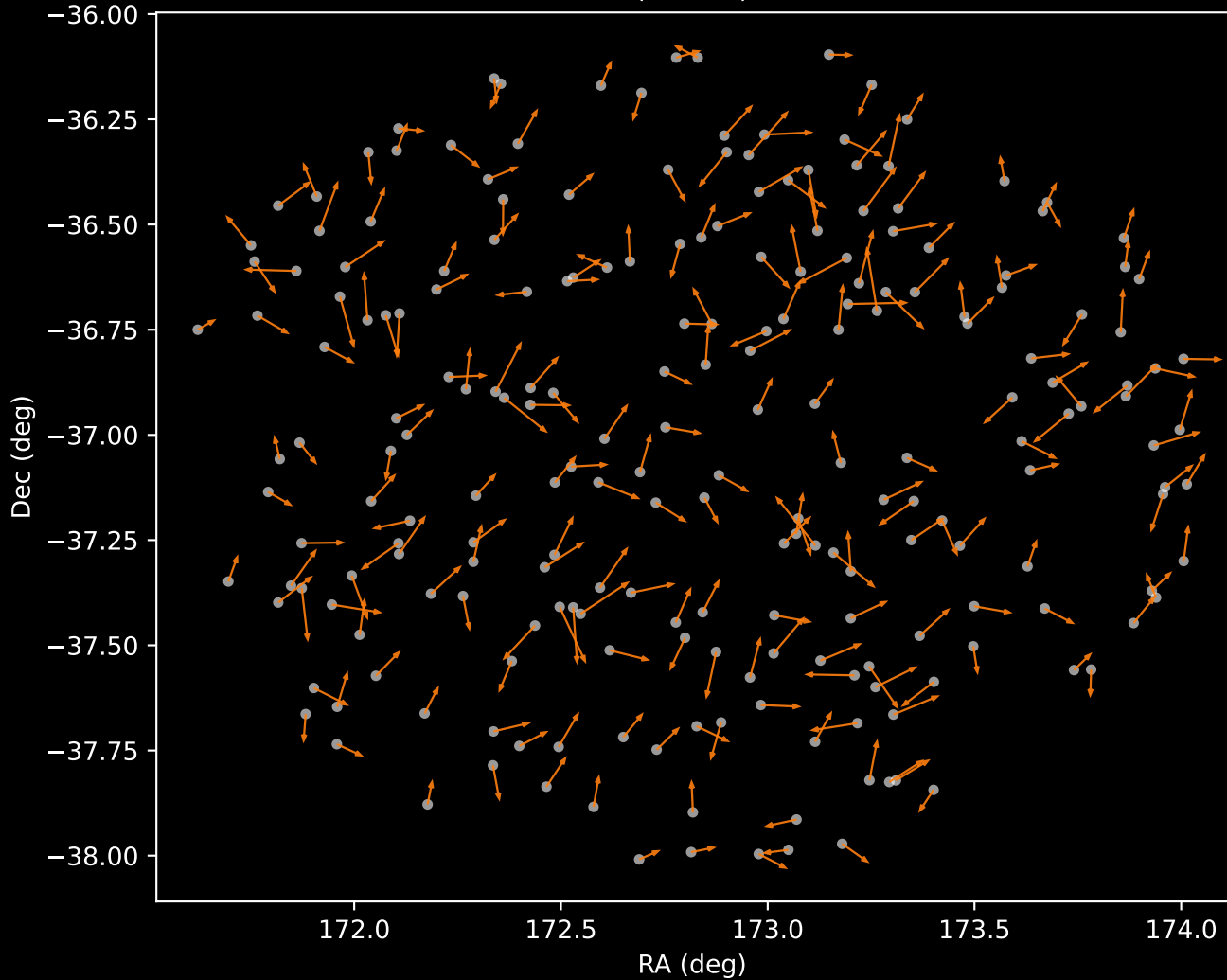
GALAH DR4 Cluster 2 Proper Motion Vectors (n=223)
