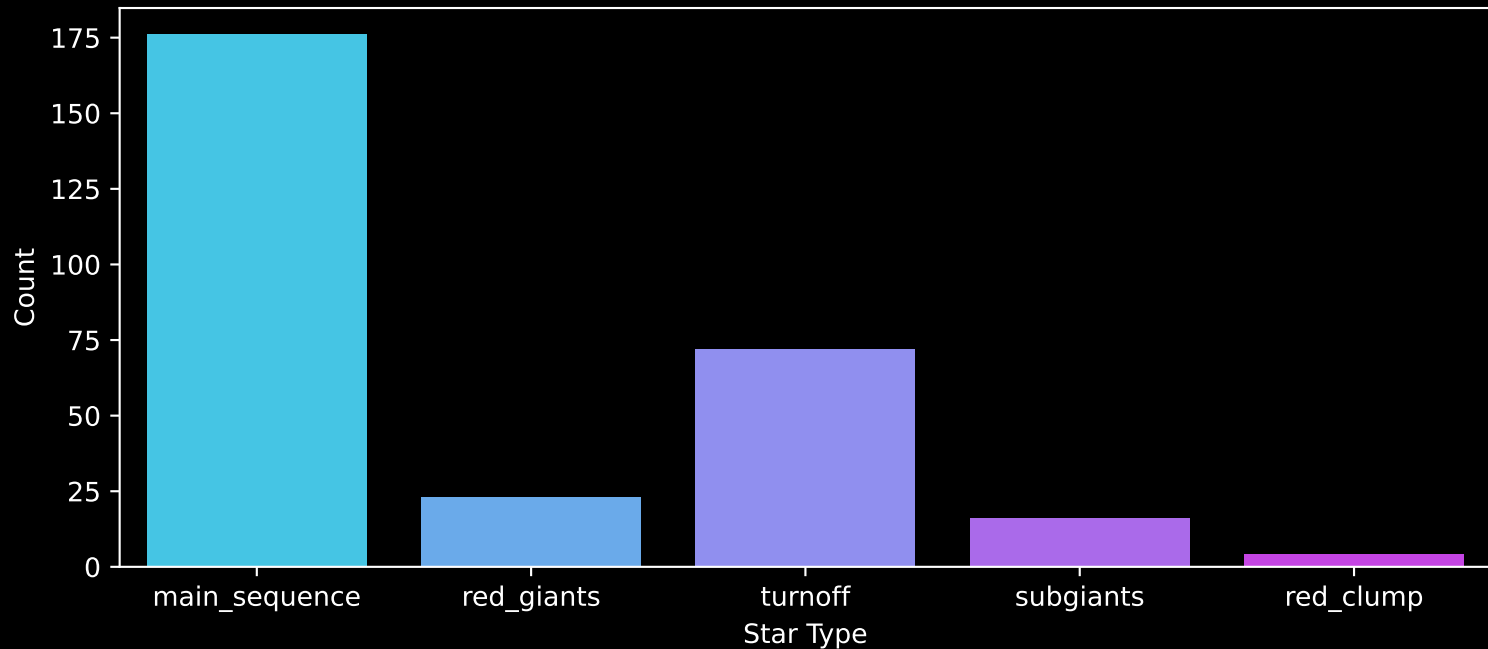
GALAH DR4 Field: [307] Count plot of Star Type
